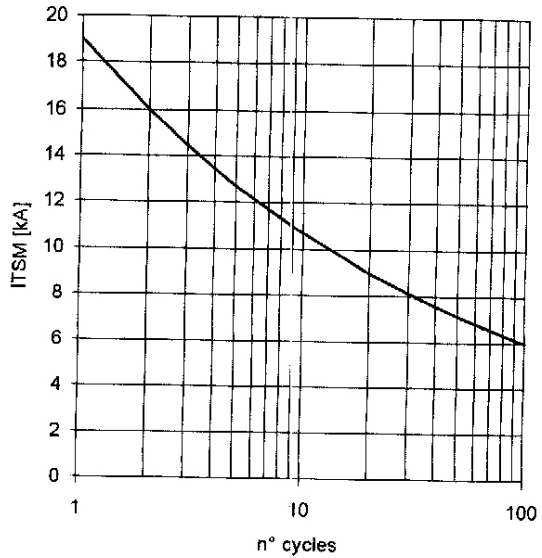
SURGE CHARACTERISTIC T j = 125 °C
