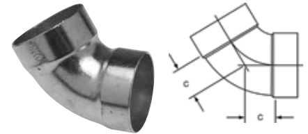
960 DWV 60° Elbow C x C – Wrot
